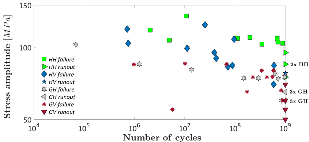
Figure 5: Experimental tests on HH, GH, HV and GV specimens: S-N plot.
