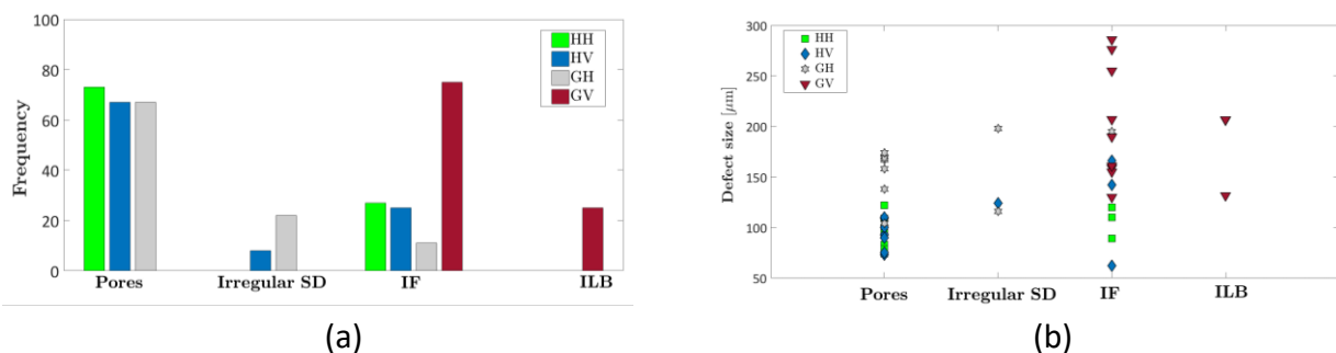
Figure 8: Defect analysis: a) frequency of occurrence; b) size of the critical defect subdivided for type and tested specimen.
