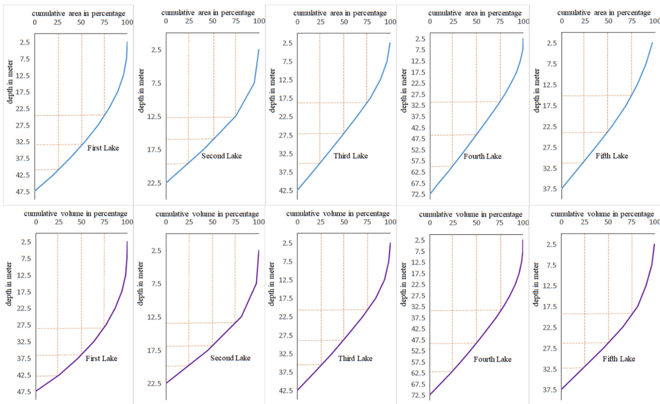
Fig. 5. Hypsographic curves for Toshka Lakes. Notice that the x-axis is located at the top of the figure in the common format for this type of graphic curve, which allows the depth measurements to be displayed in a downward direction.
