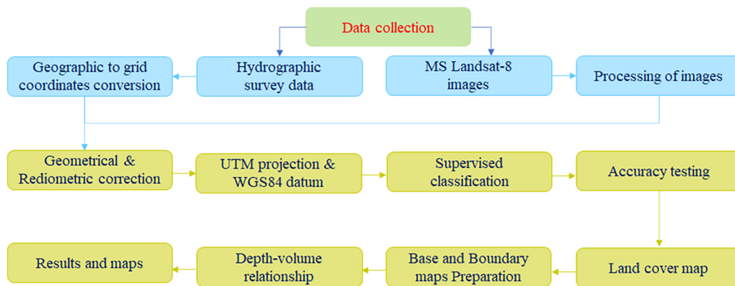
Fig. 2. Flowchart showing the processing steps used to estimate water depth, area, and volume in the Toshka Lakes.
