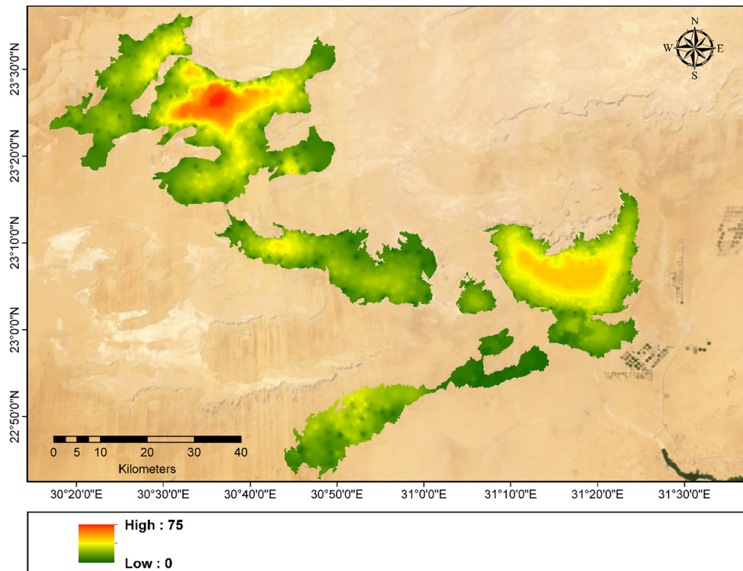
Fig. 4. Bathymetric maps of the five Toshka Lakes obtained using the proposed combination of lake bathymetric measurements, RS and GIS technologies.
