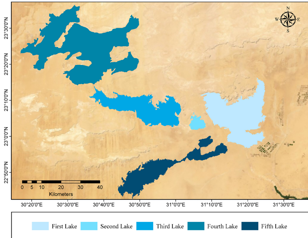
Fig. 3. The surface of the Toshka Lakes, using image satellite data (Landsat 8) and the GIS program.
