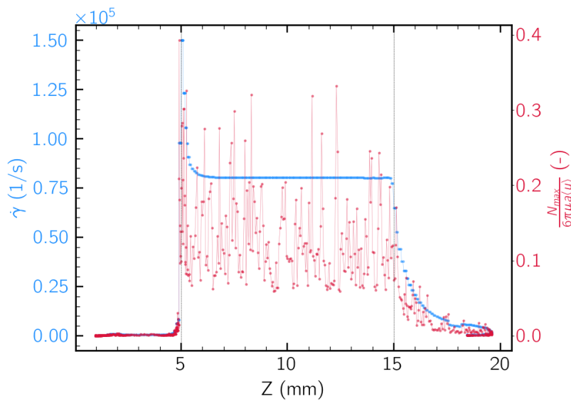
FIGURE 12 : Strain rate \dot{\gamma} (blue) and normalized maximum tensile stress N_{max} inside an isotactic cluster (red) along the Z -coordinate for a sample trajectory in the microchannel. The fluctuating behaviour of N is due to changes in the orientation of the cluster with respect to the flow field.
