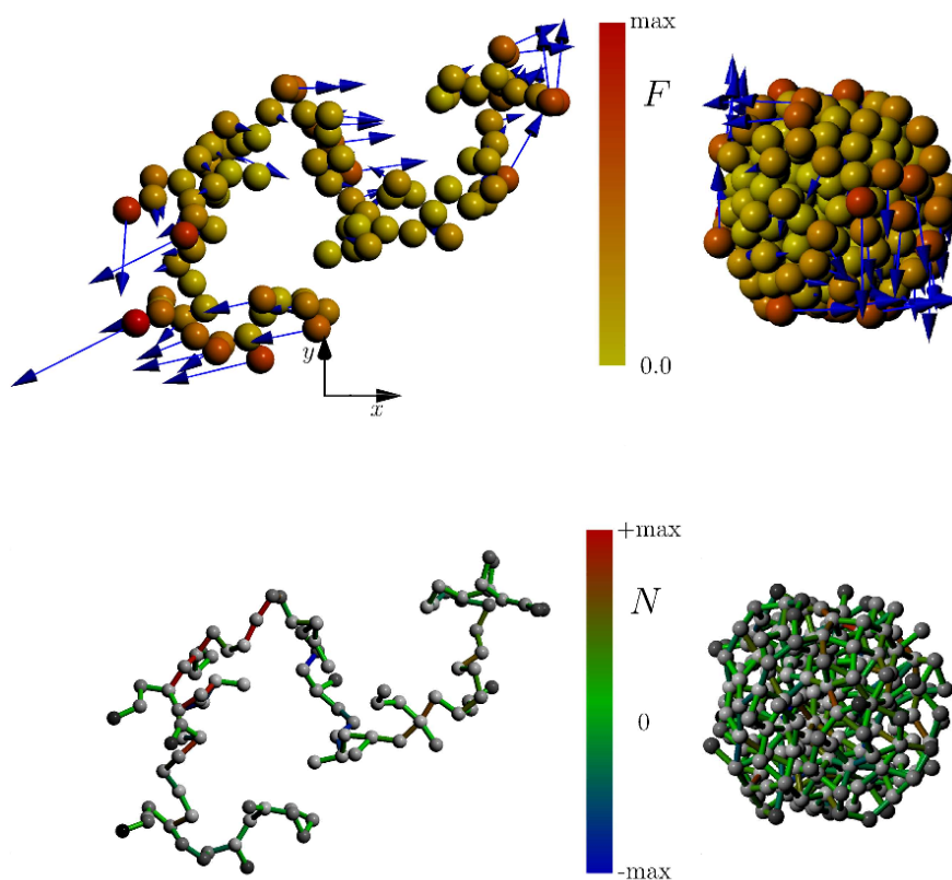
FIGURE 10 : Drag forces (above) and normal stresses at intermonomer bonds (below) for a cluster–cluster fractal aggregate (left) and random close packing (RCP) aggregate (right) under a flow with shear rate d v_x / d y
