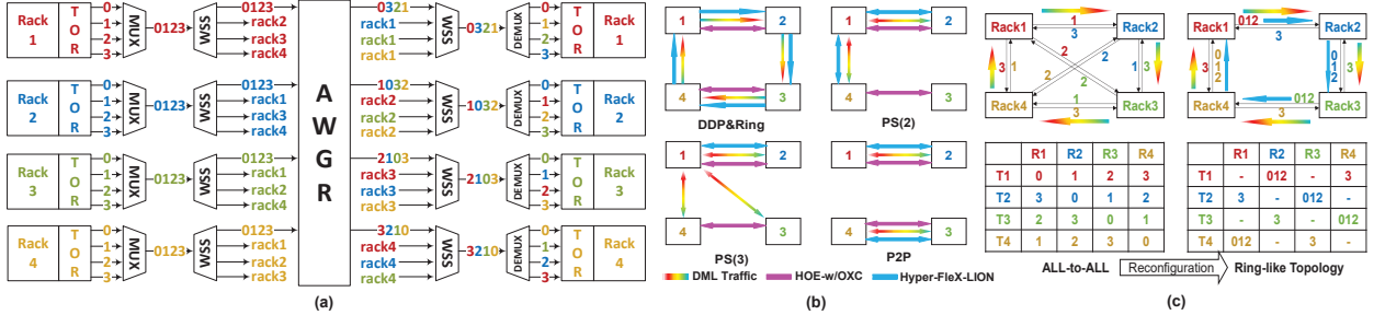
Fig. 1. (a) Hyper-FleX-LION, (b) Traffic patterns of DML architectures, and (c) Reconfiguration of Hyper-FleX-LION.
