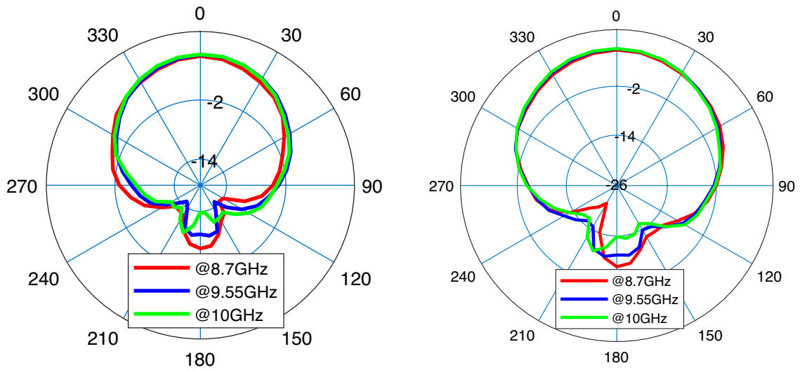
Figure 11. Radiation pattern of fabricated antenna-1 at f_1 = 8.7 GHz (red), f_2 = 9.55 GHz (blue), and f_3 = 10 GHz (green); \phi = 0^\circ (left), \phi = 90^\circ (right).
