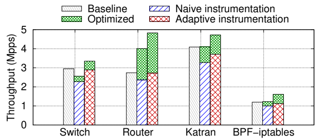
Figure 7: Naive vs adaptive instrumentation (low locality traffic). In the naive case all map lookups are recorded, while adaptive instrumentation adjusts data sampling selectively for the access patterns at each lookup call site.
