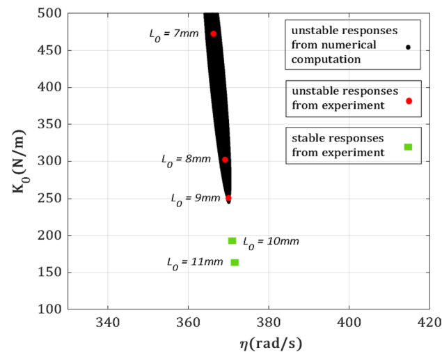
Fig. 11 Stability plot corresponding to the test rig at the combination parametric resonance frequency
