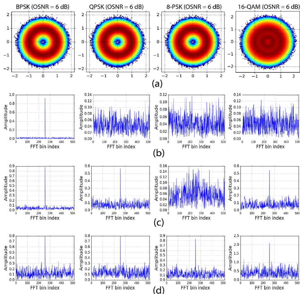
Fig. 2. (a) Constellation diagrams. (b) FFT after ()^2 . (c) FFT after ()^4 . (d) FFT after ()^8 .
