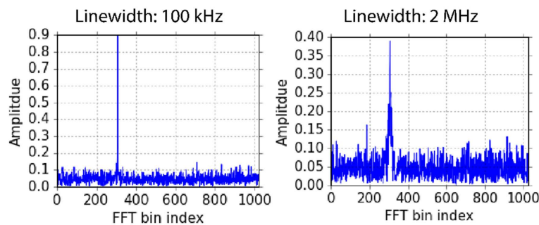
Fig. 8. Energy leakage induced from the larger phase noise for 16-QAM signal after 4th power operation.
