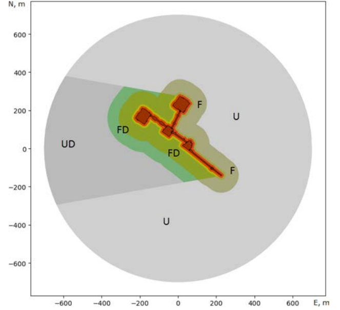
Fig. 24. Regions where the motion control is fully actuated (F, FD) and underactuated (U, UD).
