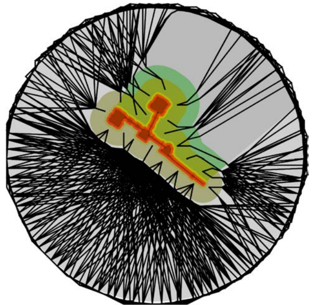
Fig. 29. Result of plotting 2000 approach trajectories with a connectivity method described in Section IV-C for the UD region, 16 neighbor node reach, \varphi_{\text{env}} = 225^\circ .
