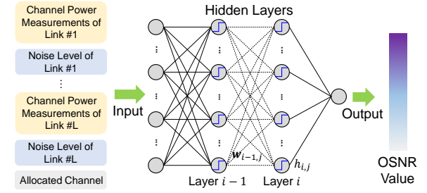
Fig. 7. Structure of the OSNR estimator.
