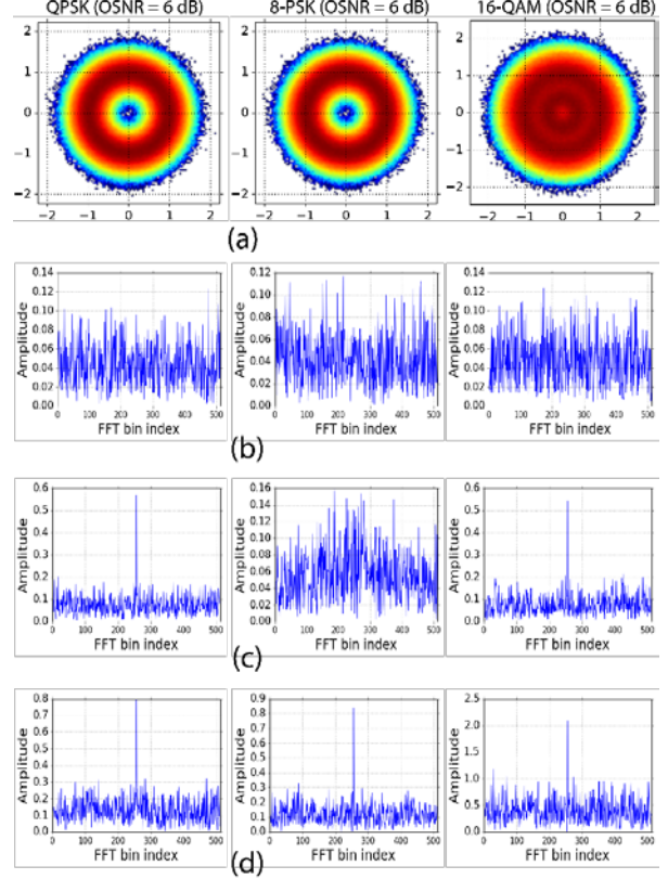
Fig. 3. (a) Constellation diagrams. (b) FFT after (\cdot)^2 . (c) FFT after (\cdot)^4 . (d) FFT after (\cdot)^8 . [9]
