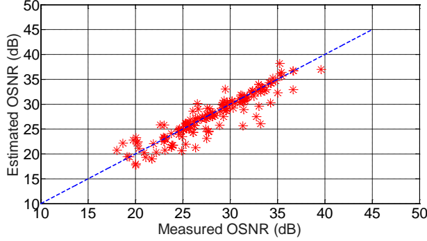
Fig. 9. Comparison between measured and estimated (red stars) OSNR.
