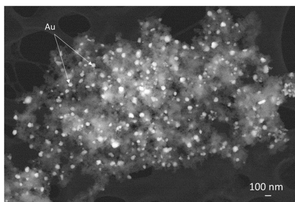
Figure 5. STEM analysis of magnetite nanoparticles decorated with Au nanoparticles using tannic acid as reducing agent.
