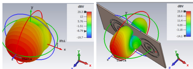
Fig. 9. Radiation pattern of the initial (left) and expanded (right) optimized FSS at 13 GHz.
