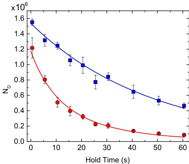
FIG. 8. Stability of a magnetically trapped Cr D -state cloud accumulated for 3 s within the MOT quadrupole, with (red circles) and without (blue squares) a {}^6\text{Li} MOT of about 2 \times 10^8 atoms and a peak density of 4 \times 10^9 atoms/cm 3 superimposed to the quadrupole center. The single Cr cloud features a dynamics that is excellently fitted by a single exponential decay, with 1/e time of \tau_D = 48(2) s (blue solid curve). The presence of the Li cloud reduces, although not dramatically the Cr 1/e lifetime to 13.0(7) s (red solid curve).
