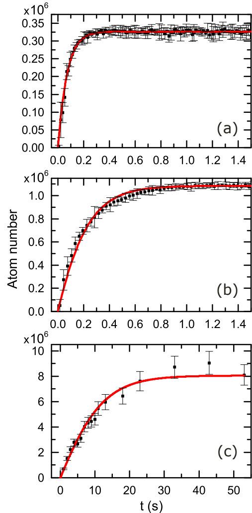
FIG. 6. (a) Loading curve of a ^{53}\text{Cr} MOT without red repumpers. Data are obtained by recording the MOT fluorescence as a function of the loading time on a CMOS camera with a 60(10) Hz frame rate. The y-axis is calibrated by independently measuring the steady-state atom number via absorption imaging. (b) Same as panel (a) , but with the red repumpers permanently on. (c) Loading curve of D -state atoms accumulated in the magnetic quadrupole and recaptured within the MOT after application of a 30-ms-long pulse of the red repumpers. The atom number is in this case monitored by means of absorption imaging. Red solid curves are the best fit to the models described in the main text.
