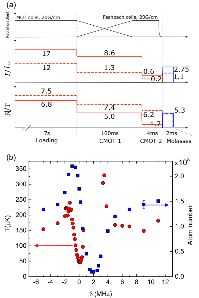
FIG. 4. (a) Sketch of the experimental routine employed to produce cold clouds of 6 Li atoms in our experiment. For each stage, red (blue) solid and dashed lines indicate the parameters exploited for D_2 ( D_1 ) cooling and repumper lights, respectively. The transfer from the MOT coils to the Feshbach coils quadrupole is also shown by the black solid lines. (b) Temperature (red circles, left axis) and atom number (blue squares, right axis) as a function of the relative detuning \delta of the D_1 repumper and cooling lights, recorded after 2 ms of gray molasses. At the Raman condition, \delta = 0 , a minimum temperature of 45(5) μK is obtained, with a cooled fraction N/N_0 \sim 70\% . For this measurement, the total cooling and repumper peak intensities were fixed to the optimum values I_{cool} = 2.75 I_{S,Li} and I_{rep} \sim 0.4 I_{cool} , respectively.
