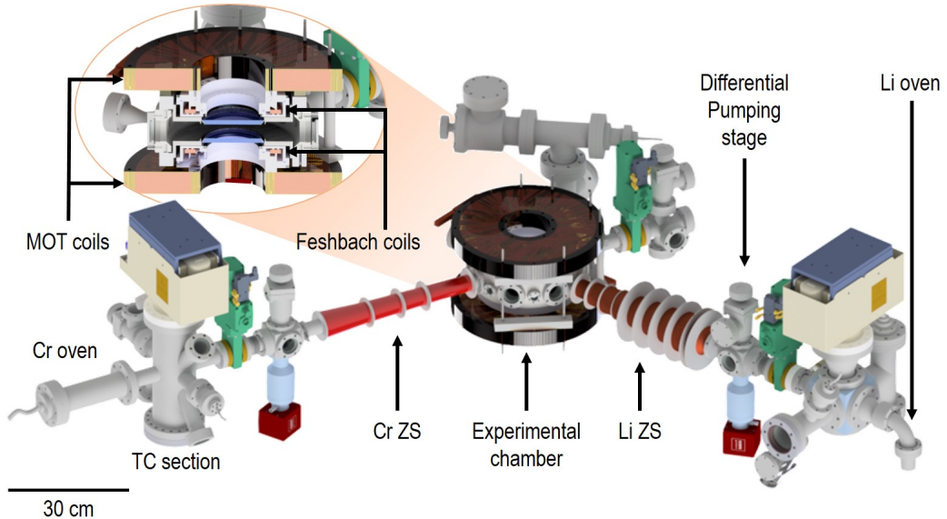
FIG. 1. Overview of our vacuum setup. Two independent ZS lines connect the Li and Cr effusion cells to a custom Kimball Physics spherical octagon chamber of radius 13 cm. In the horizontal x - y plane, the cell has 8 CF40 windows, spaced out by CF16 windows. Along the vertical z direction, two re-entrant CF200 windows with a wide clear aperture (radius 47.5 mm) ensure large optical access. Two large MOT coils, embedded within a resin structure, are fixed at the top and bottom of the science chamber, in a concentric configuration with respect to the smaller Feshbach coils, hosted within the re-entrance of the CF200 windows, see section view on the top left. The large radius of our MOT coils ensures the merging of the two ZS field profiles with the MOT quadrupole radial profile (for more details see Ref. [64]).
