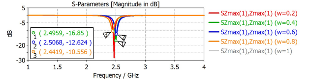
Fig. 7. Parametric variation of the trace width w of the initial design.
