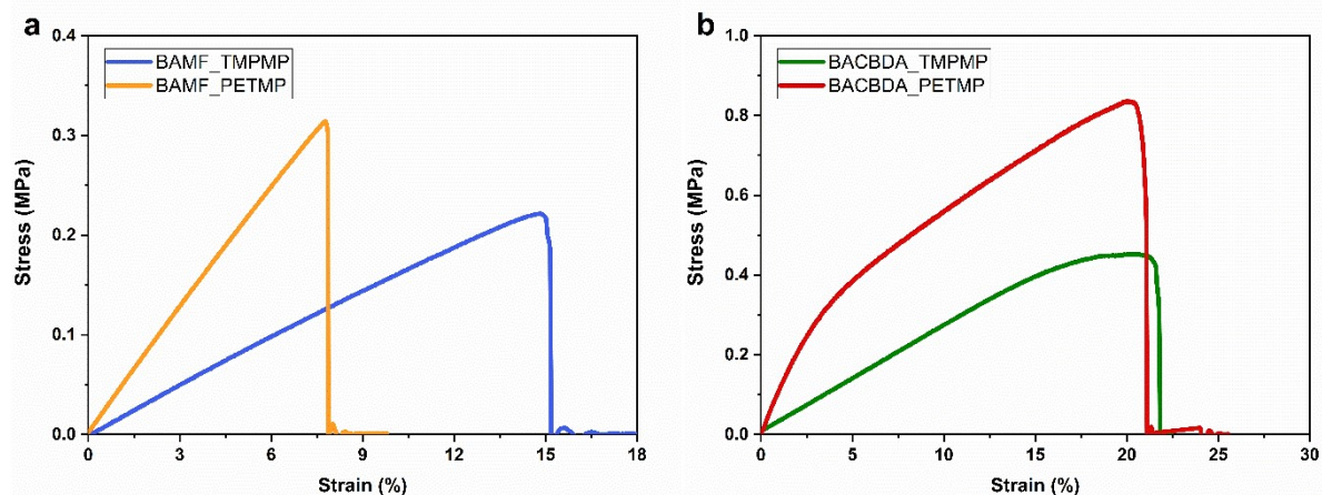
Figure 10. Stress-strain curves for the tested thermoset. (a) Thermoset bearing BAMF; (b) Thermoset produced with BACBDA as ene monomer. The reported curves were the significative ones taken from the 5-replica performed for each thermoset.
