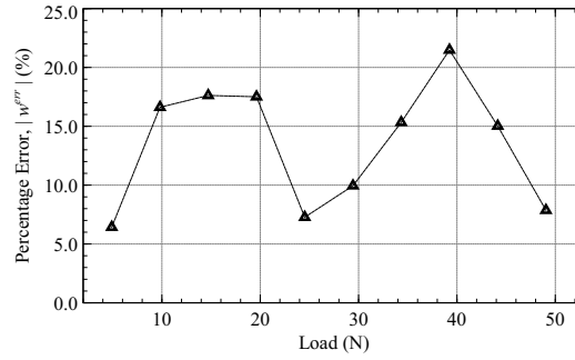
Fig. 5.24 iFEM results, obtained using one iTM2D0 element, for the metallic airfoil beam: percentage error in transverse deflection at x=0.76 L , as a function of the load applied
