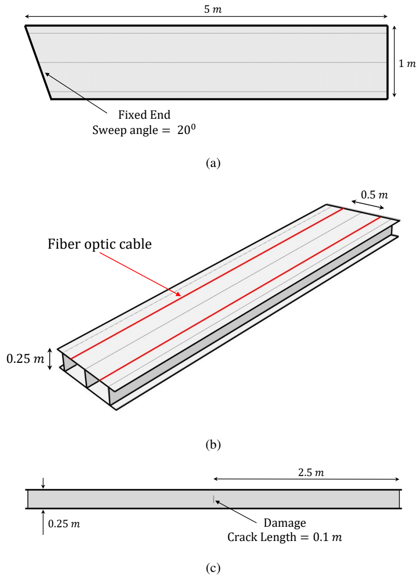
Fig. 4.32 Model of the swept wing box structure: (a) top view showing the dimensions and swept end, (b) isometric view showing the fiber optic sensors, and (c) right-side view showing the position and size of the damage
