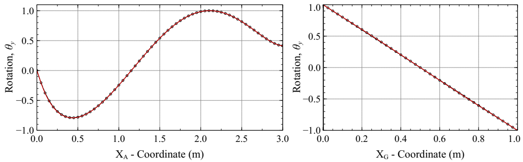
(d) Line plots of rotation, \theta_y , along sections A-A' and G-G'
