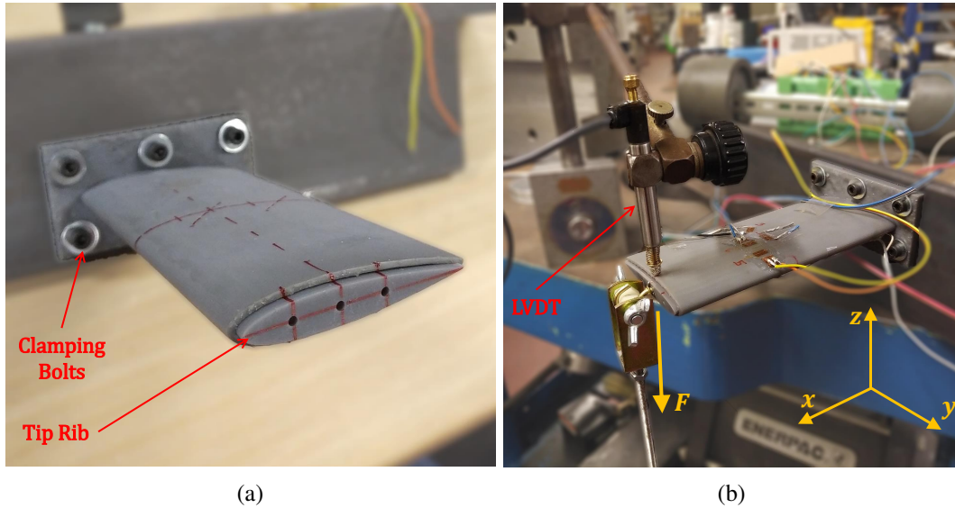
Fig. 5.13 Images of the experimental setup: (a) beam specimen clamped onto a metallic base, (b) the instrumented sensors, loading setup and LVDT locations
