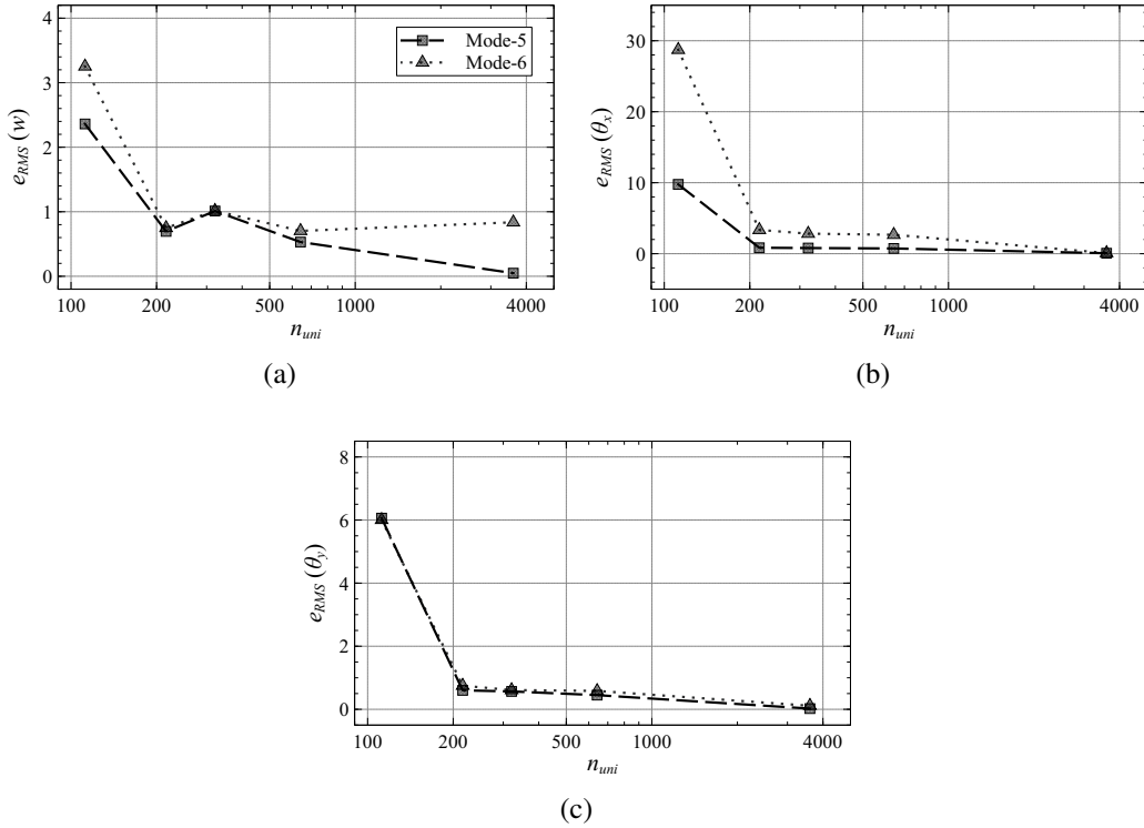
Fig. 4.14 RMS error in iFEM reconstructed (a) w , (b) \theta_x , and (c) \theta_y fields, as a function of the number of uni-axial strain measurements
