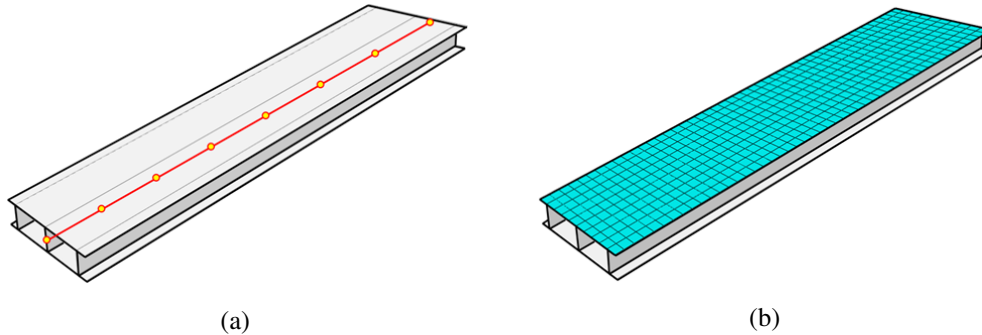
Fig. 4.33 The iFEM meshes used for wing box shape sensing: (a) discretisation using inverse beam elements (figure not representative of the actual number of elements used), and (b) top plate discretised using iQS4 elements
