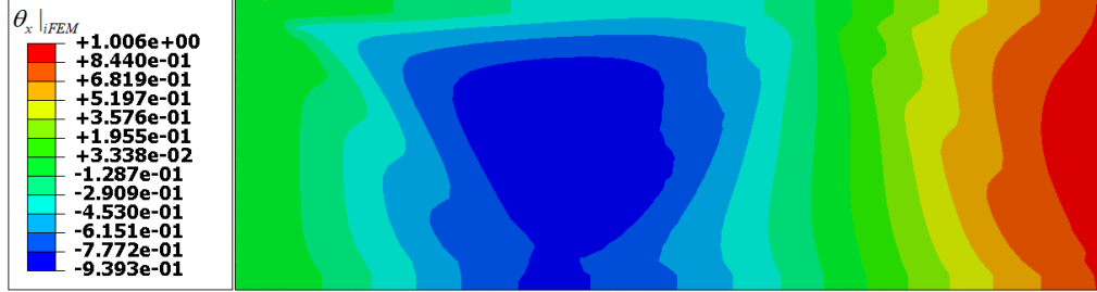
(a) Contour plot of rotation, \theta_x , for Mode 5
