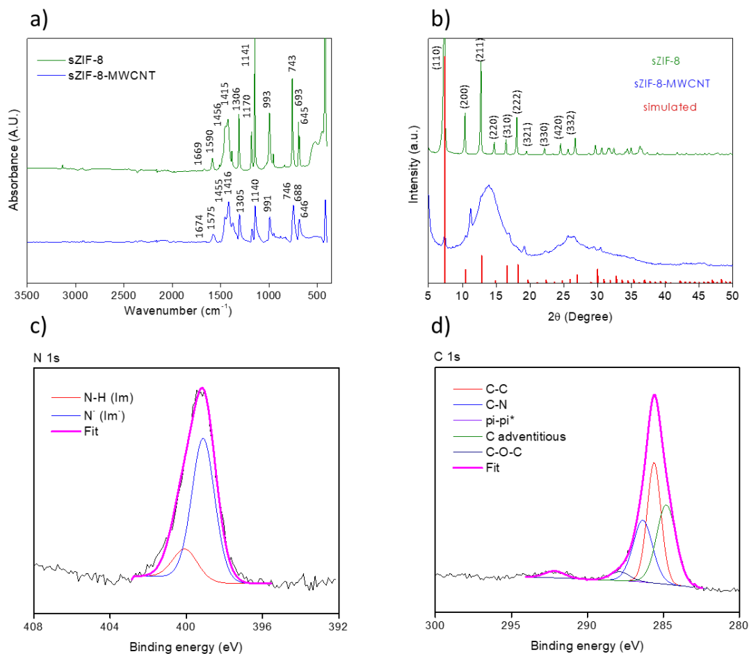
Figure 4: a) ATR spectrum of s ZIF-8 (green) and s ZIF-8-MWCNT (blue) sample. b) XRD patterns of s ZIF-8 (green), s ZIF-8-MWCNT (blue), ZIF-8 simulated (red). XPS spectra of s ZIF-8-MWCNT of c) N_{1s} and d) C_{1s} regions.
