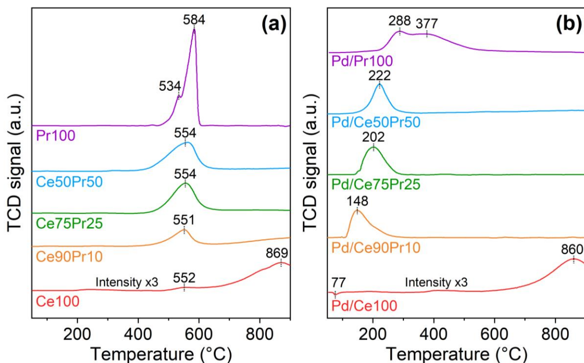
Fig. 5. H 2 -TPR profiles of supports (a) and palladium-impregnated catalysts (b) in the extended 50 – 900 °C temperature range.
