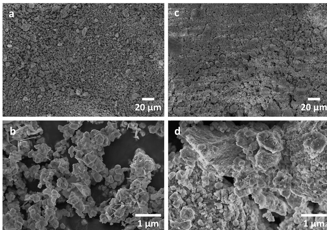
Fig. 10. FESEM morphological characterization of EoL Ni-YSZ powders before (a,b) and after (c,d) HNO 3 acid leaching.
