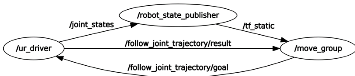
Graph 3. After application of MoveIt package on UR5
