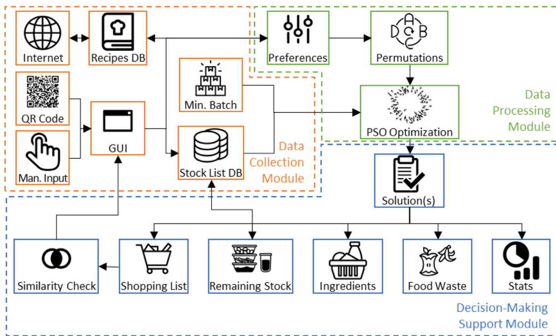
Fig. 3. Overall framework scheme.
