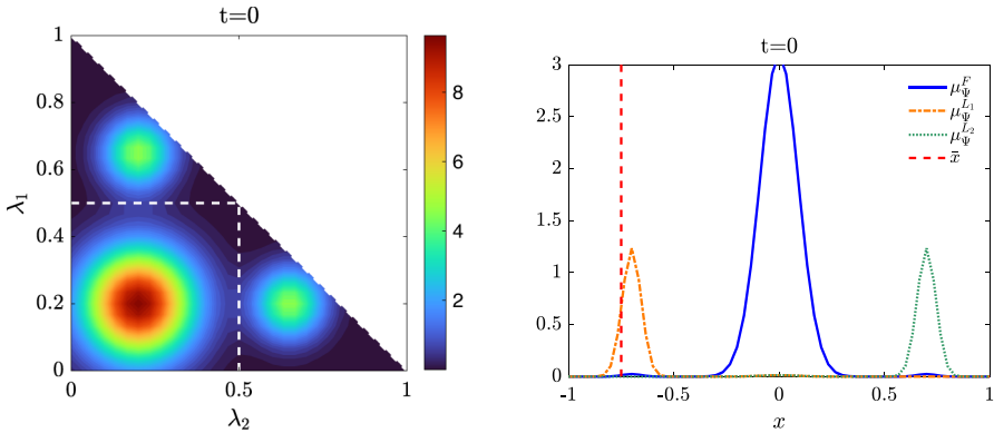
Fig. 5 Test 2. Initial distribution \Psi_0(x, \lambda) and the marginals associated with the opinion space x , \mu_\Psi^F(t, x) , \mu_\Psi^{L_1}(t, x) , and the label space (\lambda_{L_1}, \lambda_{L_2}) , \nu_\Psi(t, \lambda) . Red dashed line corresponds to the target opinion for L_1 leaders (Color figure online)
