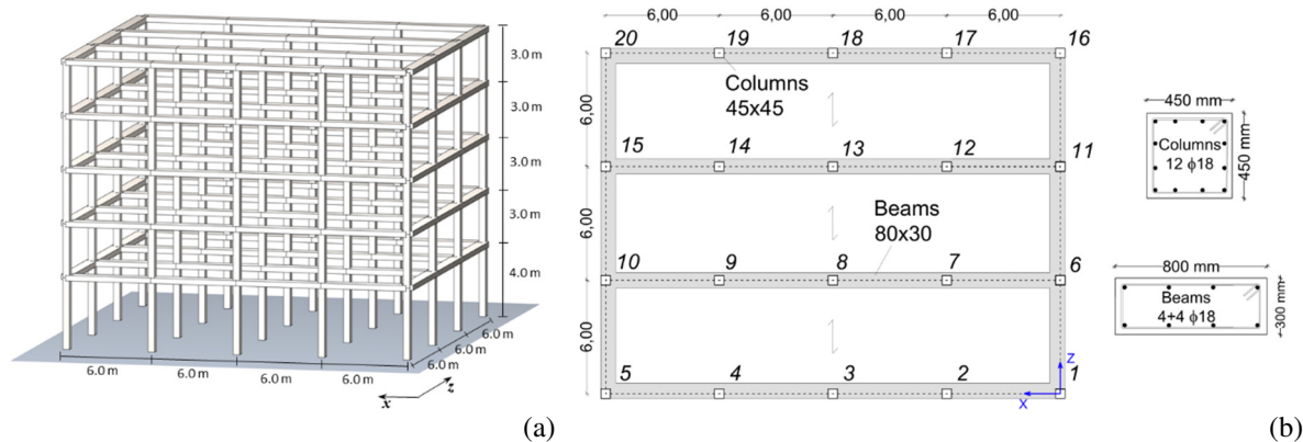
Figure 10: Geometrical dimension of the reference structural model: (a) 3D frame view; (b) in plane dimensions.
