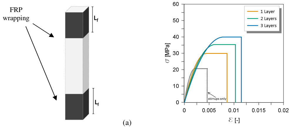
Figure 8: Details of FRP reinforcement of concrete elements: (a) Typical FRP arrangement for a column with generic confined height ( l_f ); (b) Samples of confined concrete stress–strain responses by varying the number of FRP layers.
