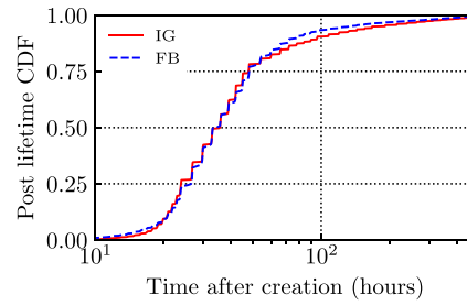
Fig. 11 Lifetime of a post computed as 95-th percentile of interactions
