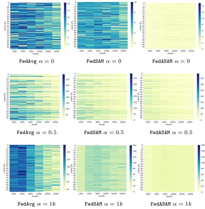
Fig. 16: Maximum Hessian eigenvalue computed for each client as rounds pass.
