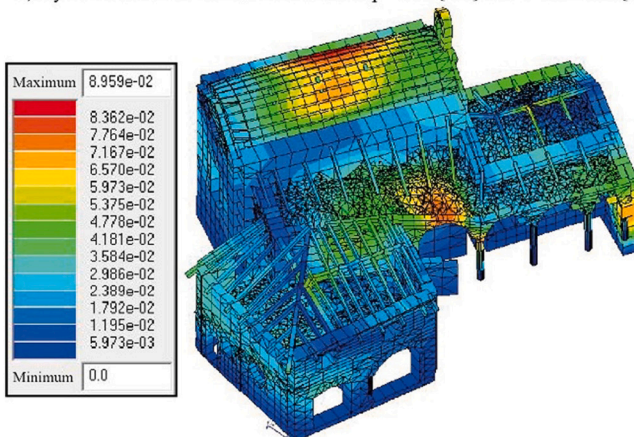
Fig. 12. Examples of results obtained in terms of deformation: maximum deformation corresponding to the static combination at Ultimate Limit State (ULS) (a). Most significant deformations deriving from the modes of vibrations for the seismic combinations (b, c, d, e).
