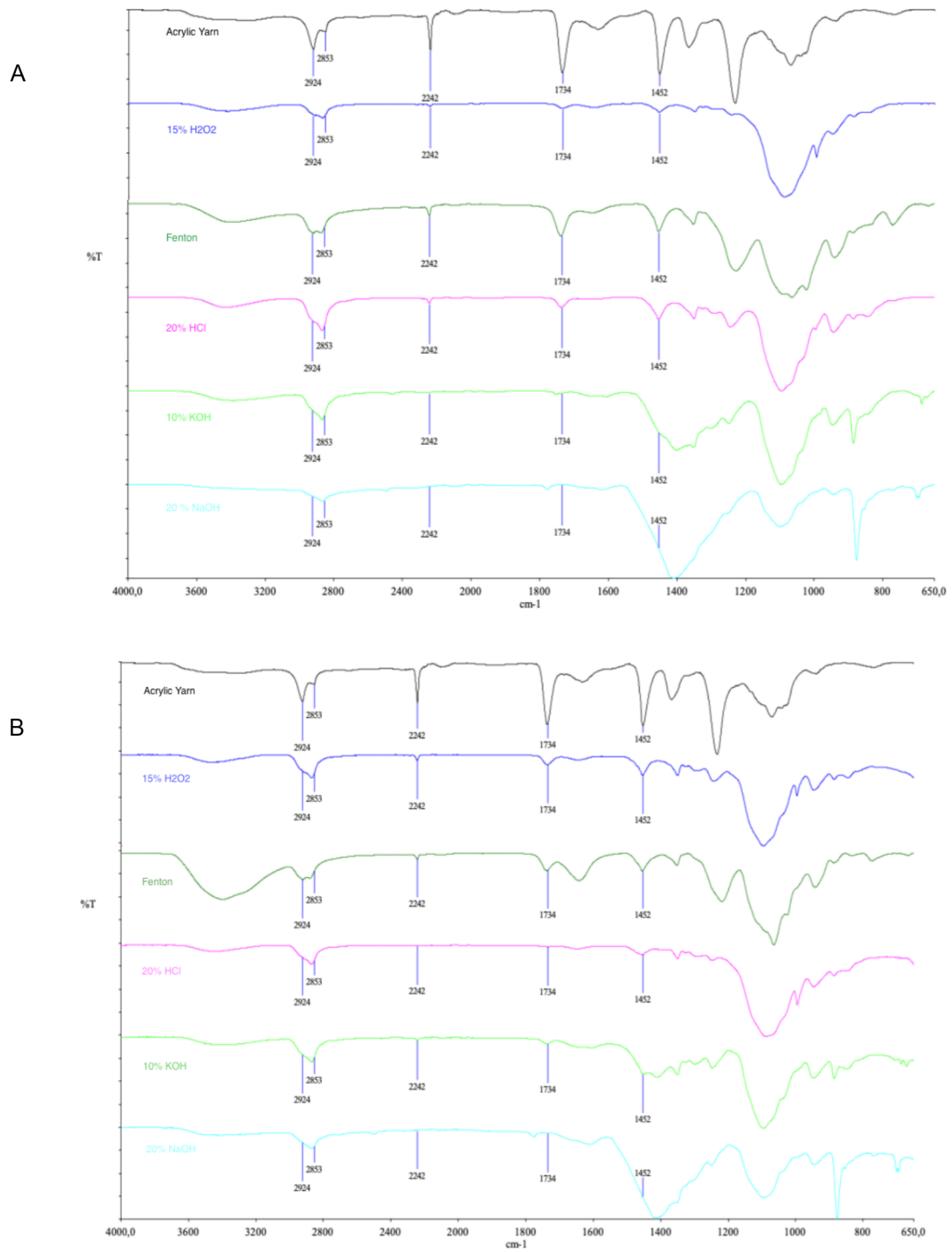
Figure 1. FTIR spectra of the MPs separated from the samples treated (A) at 25°C for 5 days, and (B) at 60°C for 6 hours
