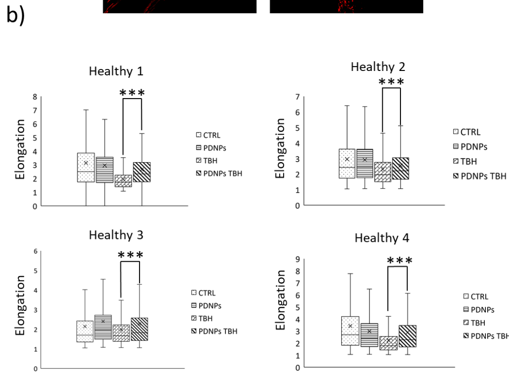
Figure 7. Analysis of mitochondrial morphology of healthy fibroblasts in different experimental conditions: a) representative confocal images; b) quantitative analysis of the elongation parameter (* p < 0.05 , *** p < 0.001 ).
