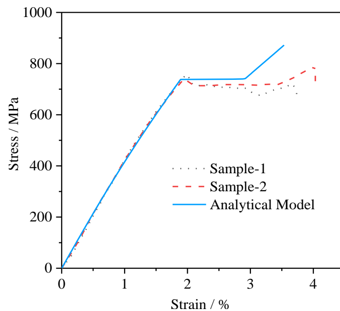
Fig. 7. Comparison of the stress-strain curves from the Fuller's tests and the analytical model.
