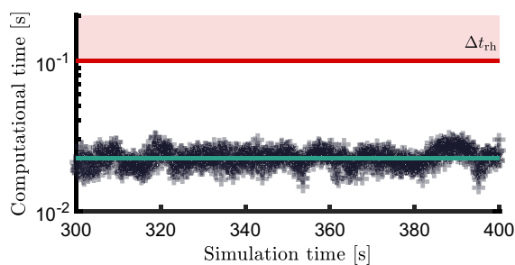
Fig. 12 Computational time required by each corresponding control calculation (indicated using ‘+’ markers) as a function of the simulation time. The solid-green line shows the average required computational time, while the solid-red line indicates the real-time limit, defined by \Delta t_{\text{rh}}
