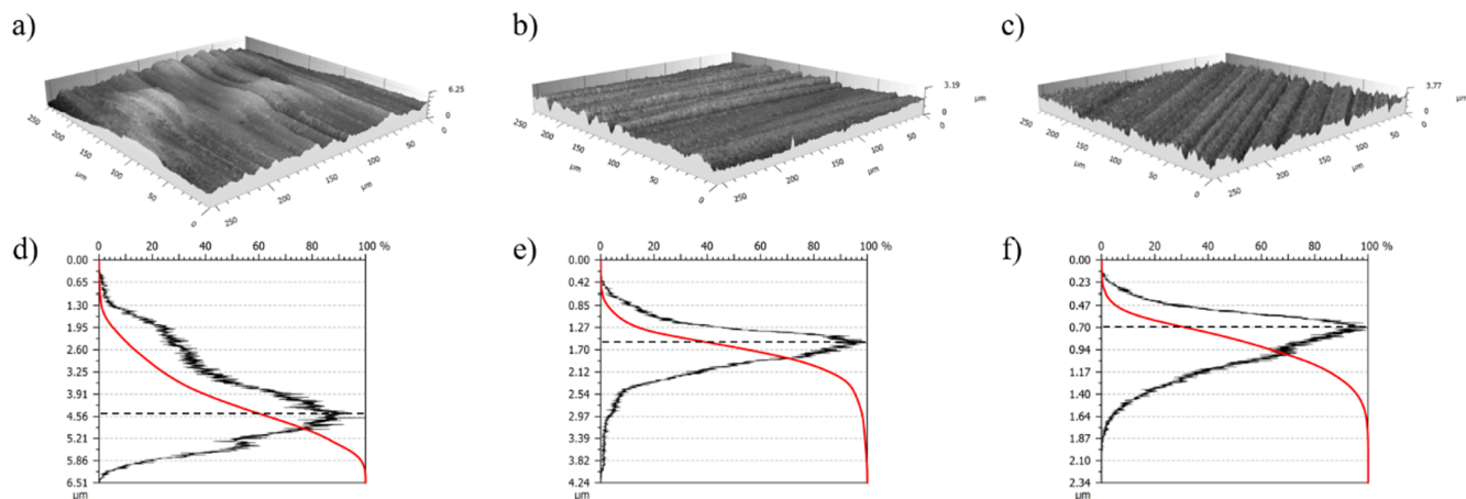
Fig. 1. 3D reconstruction images of titanium surfaces (a-c) and graphs showing the corresponding probability density function (black line) and Abbot-Firestone curve (red line)(d-e), the abscissa 0 is set at the highest point of the surface and the axis is directed downward, inside the surface: a,d) Ti(A-HC-H); b,e) Ti64(SrAg); c,f) Ti64 (HF-H 2 O 2 ). The dashed lines represent the average line of the surfaces.
