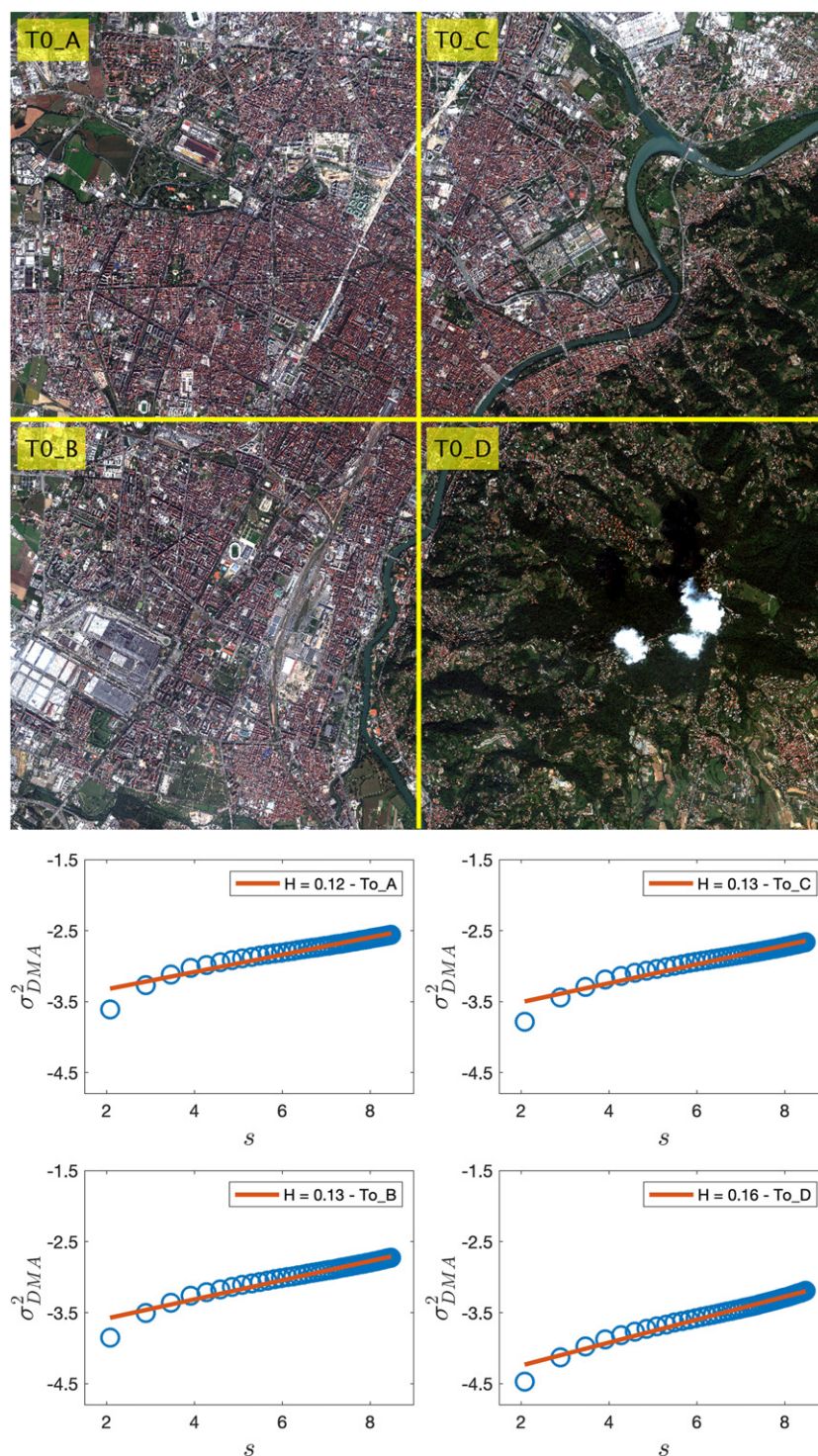
Figure 4. (Top panel) Image N45-024 (Torino) downloaded from the Urban Atlas collection of the largest European cities of WorldView-2 satellite images [40]. The image is multi-spectral with size 1080 \times 1080 . Yellow lines divide the image into four sub-images of size 540 \times 540 . (Bottom panel) Log-log plots of \sigma_{DMA}^2 for each sub-image and for the red band. Log-log axis are in natural base. Hurst exponent estimates H , obtained as the slope of the regression line by least squares, are shown for each sub-image. Goodness of fit is evaluated by R^2 provided in table 1.
