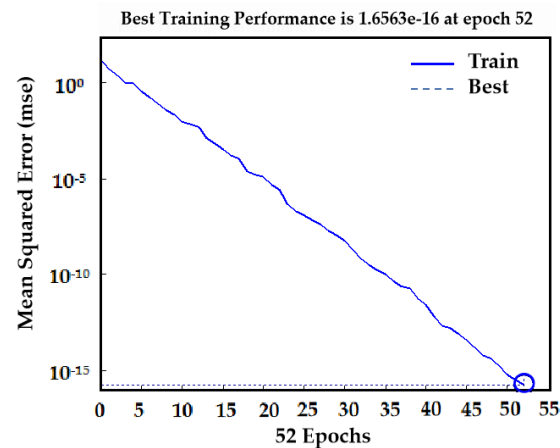
Figure 18. Multiparameter neural network training performance.
