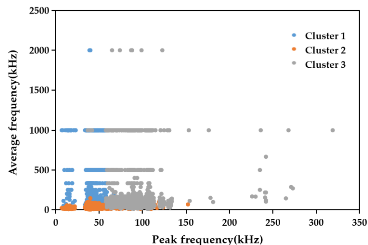
Figure 8. Density peak clustering results.
