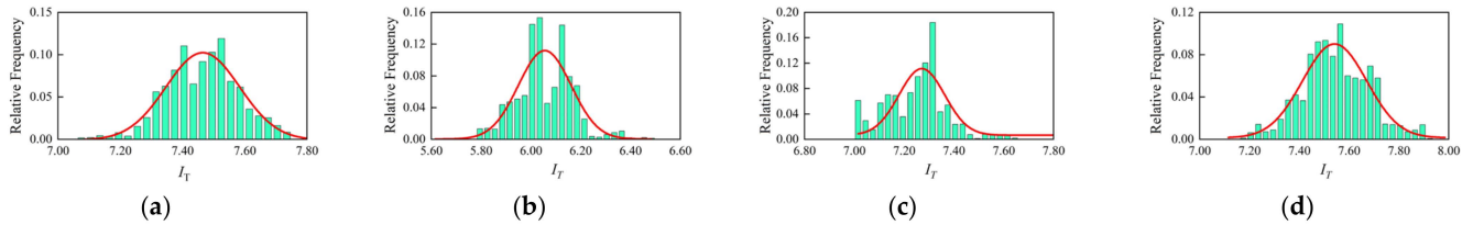
Figure 16. Posteriori relative frequency distribution of member 146. (a) Healthy; (b) failure of x -directional support restraint; (c) failure of y -directional support restraint; (d) failure of z -directional support restraint.
