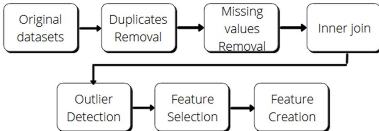
Figure 4. Adopted data pre-processing scheme.
