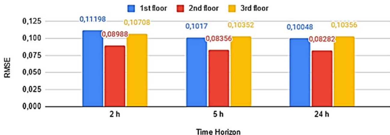
Figure 14. Average RMSE concerning time horizon by floor.
