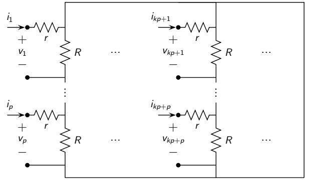
Fig. 4. Proposed regularized topology.
