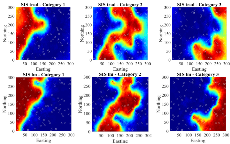
Figure 5 – Comparison of probability maps of each categories obtained by different techniques for 100 points.
