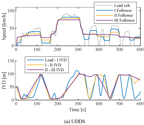
Fig. 2. Velocity profile and inter-vehicular distance IVD of the BEVs platooning in a partial time window while riding according to the urban/extra-urban drive cycles: (a) UDDS and (b) WLTP
