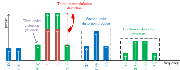
Figure 2. Third-order intermodulation distortion and products.
