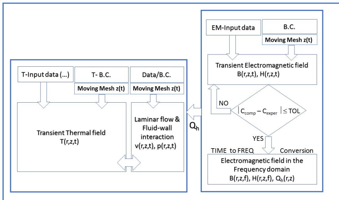
Figure 3. Field (module) coupling and Multiphysics flow of the finite element EC damper model.
