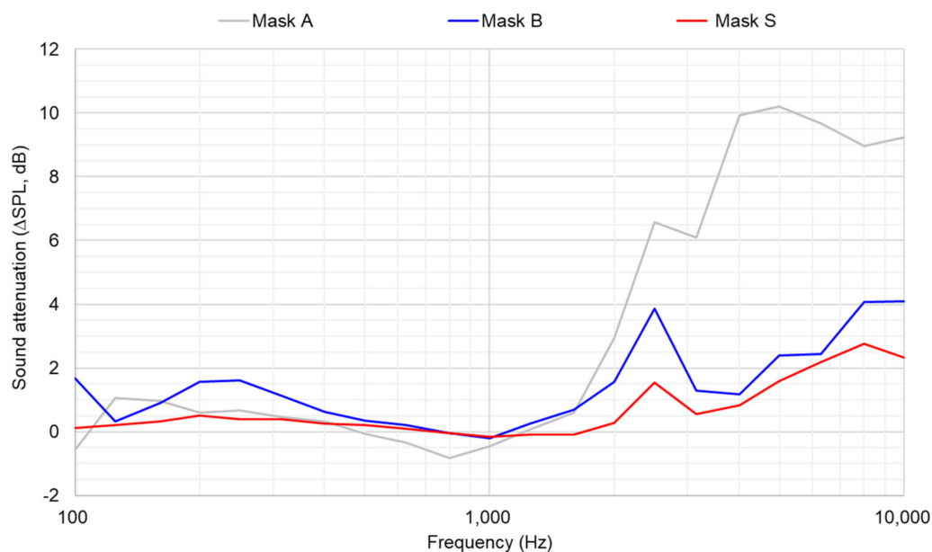
Figure 5. Spectral distribution of sound attenuation ( \Delta SPL) for the three face masks.
