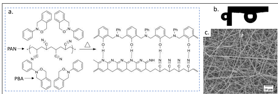
Figure 27. a. Chemical structure of polybenzoxazine/polyacrylonitrile (PBA/PAN) and intermolecular hydrogen bonding between hydroxyl groups of PBA chains and PAN after curing; b. superhydrophobic surface of electrospun membrane of PAN/PBA (50:50) with high water adhesion characteristics; c. SEM image of electrospun membrane of PAN/PBA. Adapted with permission from ref [290].
