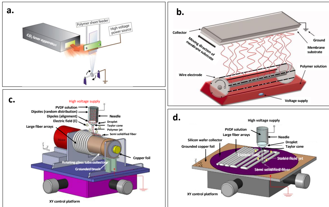
Figure 5. Schematic representations of peculiar set-ups for PVDF electrospinning. a. Melt electrospinning configuration using a \text{CO}_2 laser system. Adapted with permission from ref [42]. b. Needleless electrospinning set-up. Adapted with permission from ref [63]. c. and d. Near-field electrospinning (NFES) by drum-like collector (c) and XY stage (d). Adapted with permission from ref [61].
