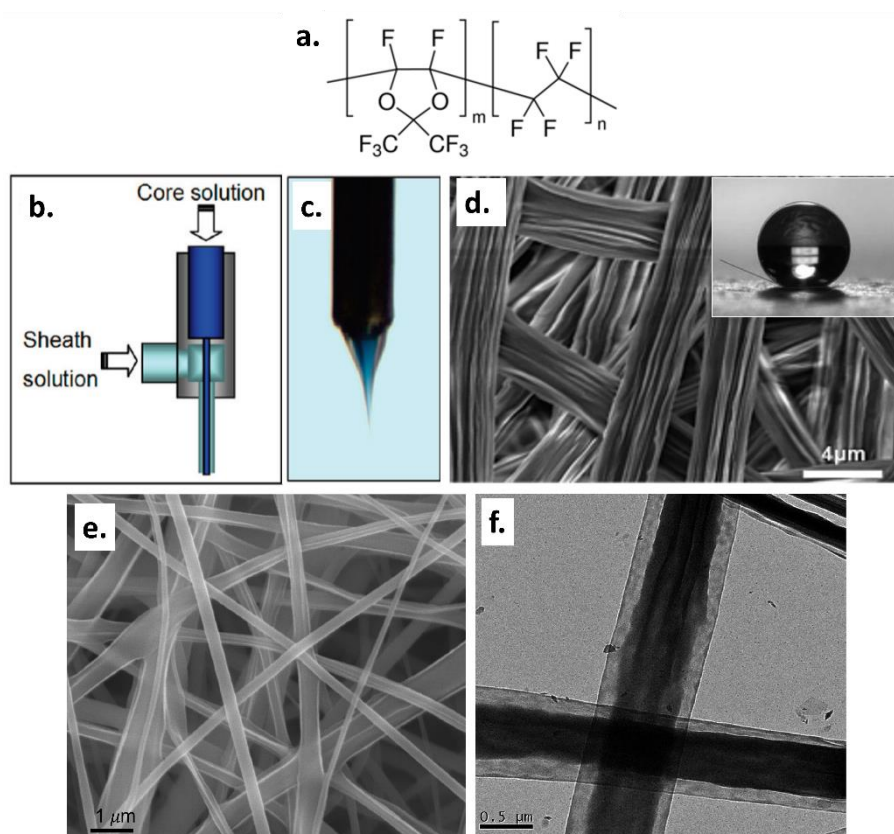
Figure 11. Teflon TM AFs electrospinning. a. Molecular structure of poly[4,5-difluoro-2,2-bis(trifluoromethyl)-1,3-dioxole- co -tetrafluoroethylene] copolymer. b. Schematic representation of the co-axial electrospinning set-up; c. Taylor cone formation for PCL/Teflon TM AF core-shell droplet; d. morphology of core-shell PCL/Teflon TM AF fibers obtained with PCL concentration of 10 wt.% and 1.5 ml/h feed rate, and Teflon TM AF concentration of 1 wt.% and 1 ml/h feed rate. Adapted with permission from ref [149]. e. and f. SEM and TEM micrographs of core-shell PVDF/Teflon TM AF electrospun fibers (PVDF solution concentration of 15 wt.% with feed rate of 0.25 ml/h; Teflon TM AF solution concentration of 1 wt.% with feed rate 0.23 ml/h). Adapted with permission from ref [150].
