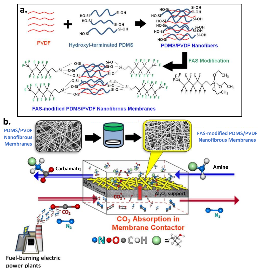
Figure 20. a. Schematic representation of FAS-modified PDMS/PVDF nanofibrous membranes preparation, b. CO 2 gas absorption in the hydrophobic membrane contactor. Adapted with permission from ref [218].
