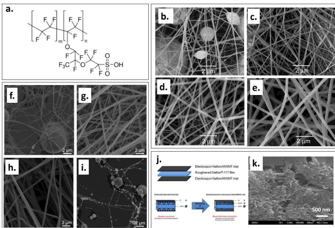
Figure 12. Examples of Nafion™ electrospinning. a. Molecular structure of Nafion™. b-e. SEM images of electrospun fibers of Nafion™/PAA with PAA content of 8 % (b), 12 % (c), 25 % (d), 66 % (e). Adapted with permission from ref [160]. f-h. SEM images of high-purity Nafion™ nanofibers, electrospun with high molar mass PEO ( M_w = 8000 kg/mol) at fiber compositions of 98 (f), 99 (g), 99.9 (h) wt. % Nafion™; i. solutions with lower molar mass PEO ( M_w = 400 kg/mol) produced beaded fibers at 99.9 wt. % Nafion™. Adapted with permission from ref [155]. j. Schematic representation of the fabrication of multilayer composite membrane actuators; k. SEM image of cross-section of the fabricated actuator. Adapted with permission from ref [164].
