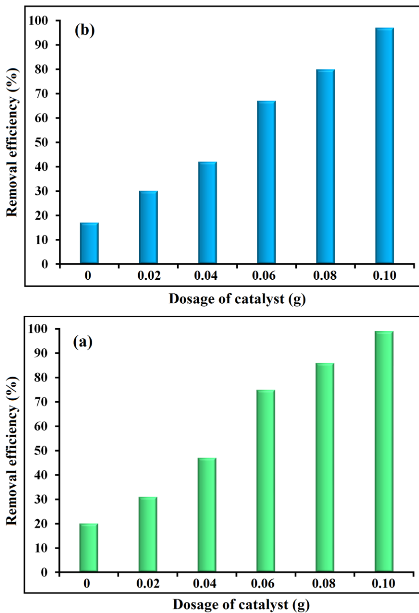
Fig. 5. Effect of (TBA)_4PW_{11}Fe@TiO_2@PVA catalyst dosage on the ODS process of (a) DBT and (b) sulfur content of gas oil.
