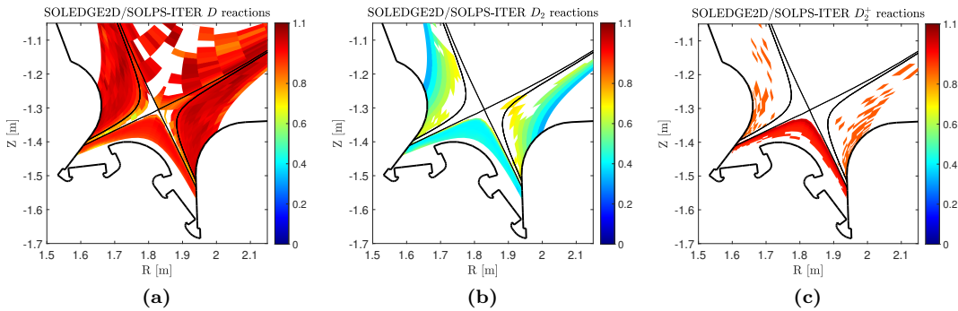
Figure 15: Cell-by-cell ratio between SOLEDGE2D and SOLPS-ITER reaction rates involving atoms (a), molecules (b) and molecular ions (c) as computed via the respective fits for the reactivities (Table 1). Density and temperature data employed are those of SOLPS-ITER.
