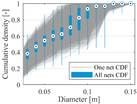
(A) Statistical distributions of diameters
