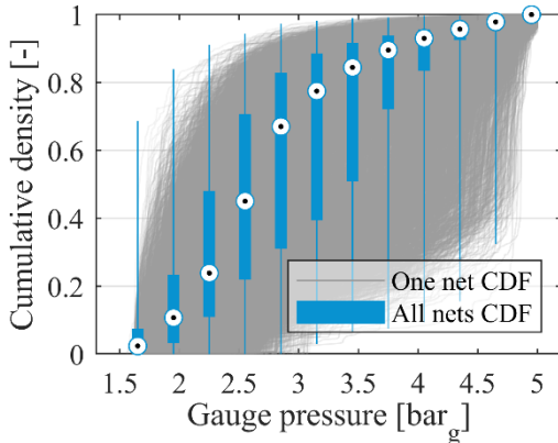
(C) Statistical distributions of nodal pressures
