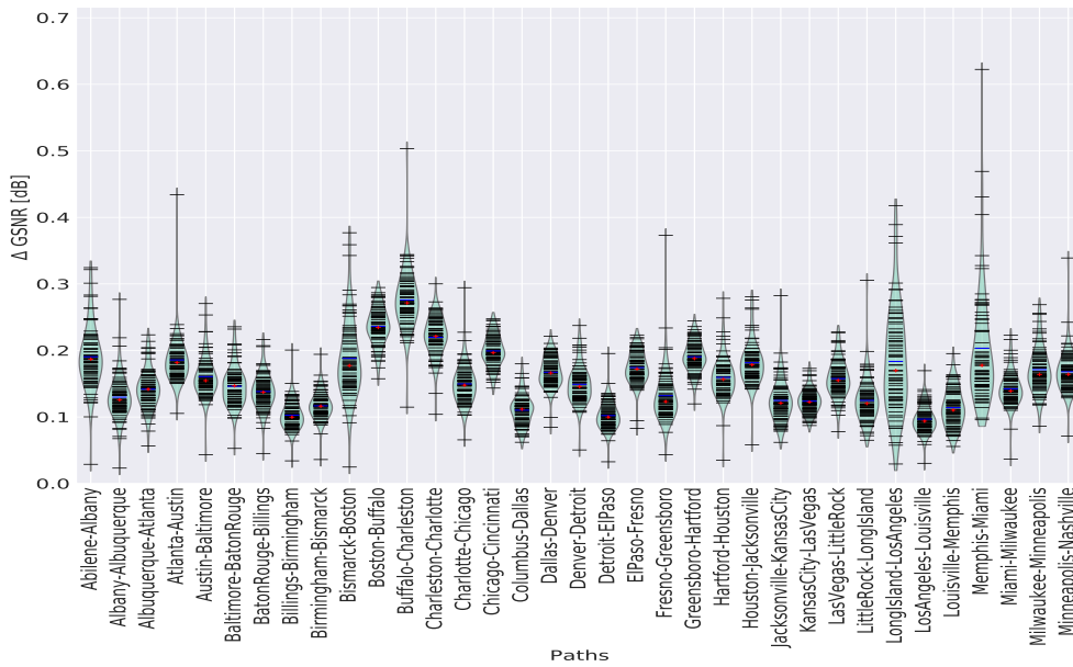
Fig. 3.14 Distribution of \Delta GSNR for the simulated links of USA network using MLPR
