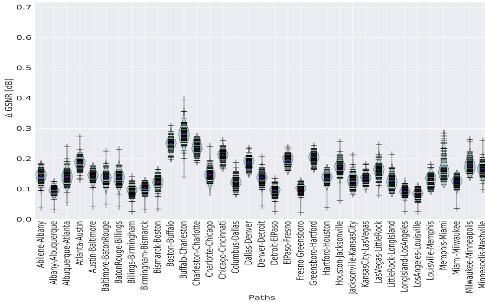
Fig. 3.16 Distribution of \Delta GSNR for the simulated links of USA network using wdnm
