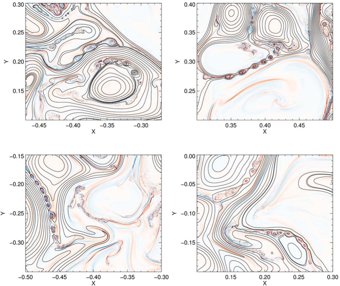
Figure 3. Zoomed-in regions of the domain in which J , at t/\tau_{nl} = 2.62 , is plotted with the corresponding magnetic surfaces, highlighting the plasmoid chains.
