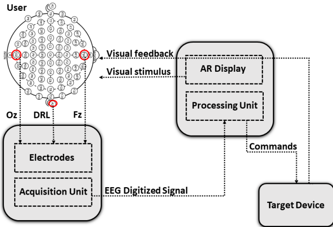
Fig. 1: General architecture of the AR-BCI SSVEP instrumentation.
