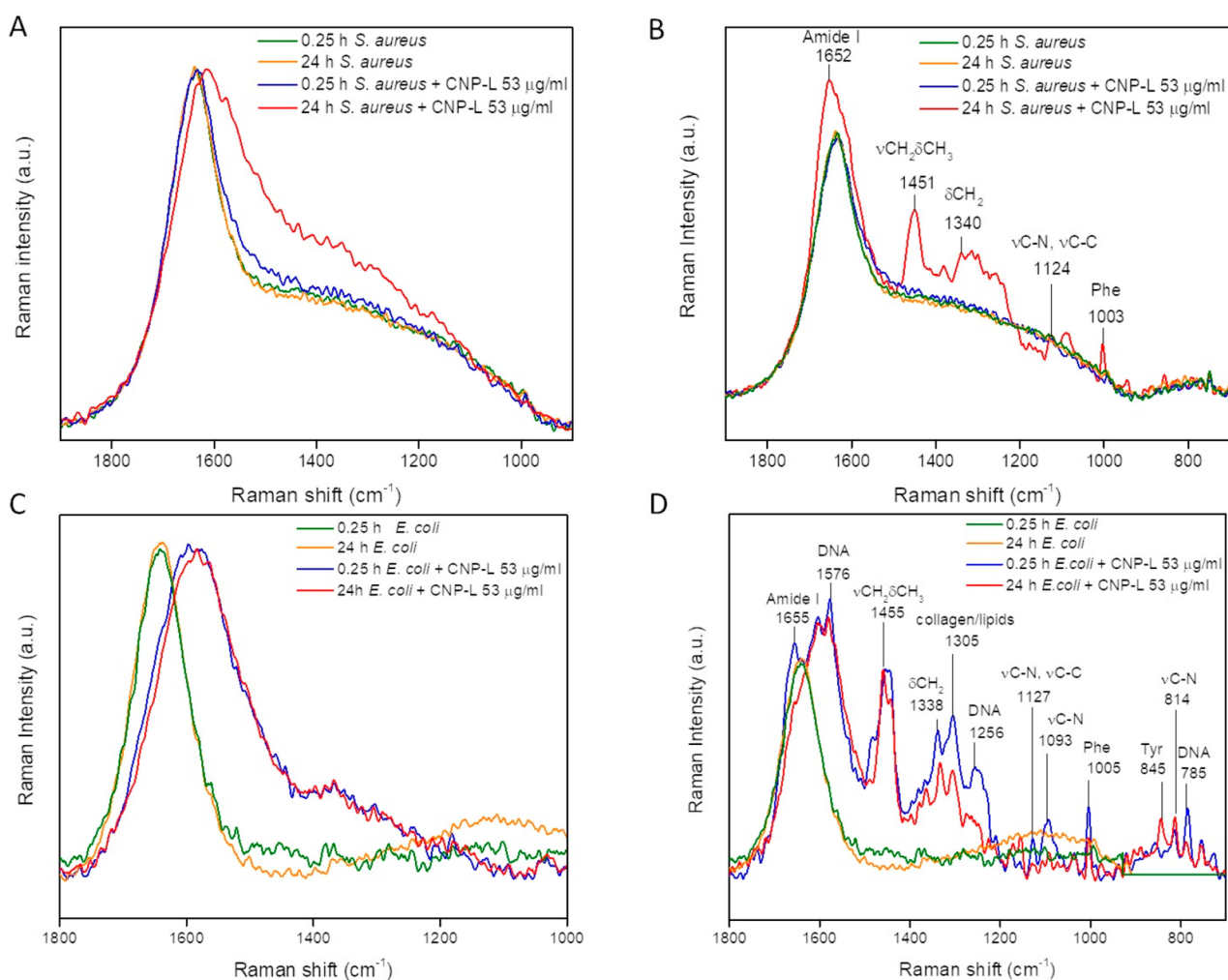
Figure 3. DEP–Raman analysis of the interaction of CNP-L with S. aureus and E. coli . DEP–Raman spectra of (A, B) S. aureus SH1000 and (C, D) E. coli MG1655 in the absence or presence of CNP-L (53 \mu\text{g}/\text{mL} ) after 0.25 and 24 h of incubation. For each bacterial strain two different signals were recorded, focalizing the Raman microscope in regions of the same sample in which the ECM was (B, D) or was not (A, C) present. Each line represents the normalized average of three Raman spectra recorded during three independent experiments.
