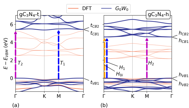
Figure 3. Band structures of \sqrt{3} \times \sqrt{3} gC_3N_4 -t (a) and gC_3N_4 -h (b), computed at the DFT (thin red lines) and at the G_0W_0 (blue lines) levels of approximation. The dashed vertical arrows mark the electronic transitions contributing to some exciton states obtained by solving the BSE. The arrows in panels (a) and (b) correspond to the crosses in the upper panels of Figure 4a and Figure 4b, respectively.
