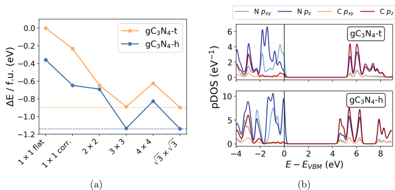
Figure 2. (a) Energy per formula unit (f.u.) of gC_3N_4 -t and gC_3N_4 -h in different simulation cells, referenced to flat 1 \times 1 gC_3N_4 -t. (b) Projected density of states of gC_3N_4 -t (top panel) and gC_3N_4 -h (bottom panel).
